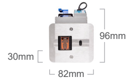
LX PRINTHEAD FRONT ELEVATION
